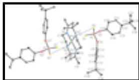
Fig. 1. The molecular structure of the title complex, showing the atom-numbering scheme with displacement ellipsoids at 50% probability level. H atoms on N are represented as small spheres of arbitrary radii and H atoms on C have been omitted for the sake of clarity. Atoms with the superscript i are generated by the symmetry operation (-x, -y + 1, -z + 1) .
